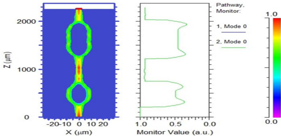
Figure 4: Simulation Effects of a double ring micro-ring resonator in Slab Mode.
