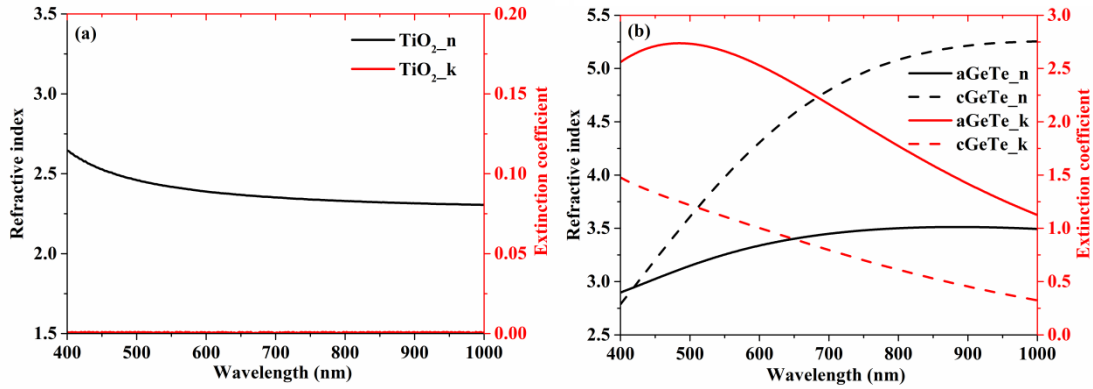
Fig.2 Optical constants (n and k) of (a) \text{TiO}_2 ; (b) amorphous and crystalline GeTe thin films (labeled as aGeTe and cGeTe), which is obtained from Ref. 26-28 .
