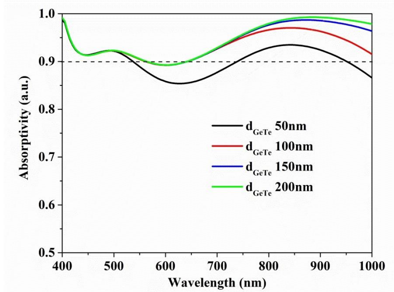
Fig.7 Absorption spectra of the designed absorbers with various thicknesses of amorphous GeTe thin films
