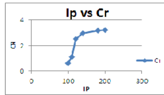
Figure 1.7: Effect of Peak current on Cutting Rate.
