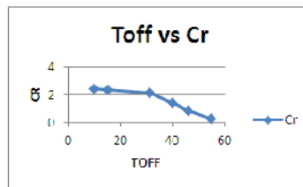
Figure 1.6: Effect of Pulse off Time on Cutting Rate.
