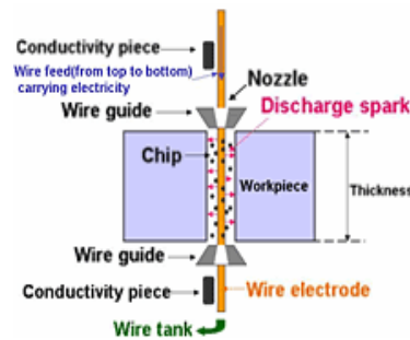
Fig 1.1: Mechanism Of Material Removal In Wedm
