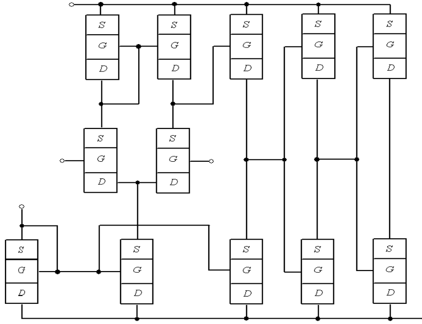
Fig. 1. The considered comparator circuit [4]
