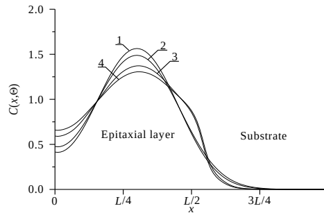
Fig. 2b. Dependences of concentration of dopant, implanted in heterostructure from Figs. 1, on coordinate in direction, which is perpendicular to interface between epitaxial layer substrate. Difference between values of dopant diffusion coefficient in layers of heterostructure increases with increasing of number of curves. Value of dopant diffusion coefficient in the epitaxial layer is larger, than value of dopant diffusion coefficient in the substrate. Curve 1 corresponds to homogenous sample and annealing time \Theta = 0.0048 (L_x^2 + L_y^2 + L_z^2)/D_0 . Curve 2 corresponds to homogenous sample and annealing time \Theta = 0.0057 (L_x^2 + L_y^2 + L_z^2)/D_0 . Curves 3 and 4 correspond to heterostructure from Figs. 1; annealing times \Theta = 0.0048 (L_x^2 + L_y^2 + L_z^2)/D_0 and \Theta = 0.0057 (L_x^2 + L_y^2 + L_z^2)/D_0 , respectively
