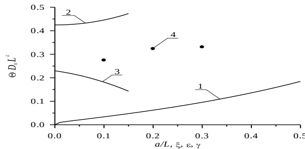
Fig. 5a. Dimensionless optimal annealing time of infused dopant as a function of several parameters. Curve 1 describes the dependence of the annealing time on the relation a/L and \xi = \gamma = 0 for equal to each other values of dopant diffusion coefficient in all parts of heterostructure. Curve 2 describes the dependence of the annealing time on value of parameter \varepsilon for a/L=1/2 and \xi = \gamma = 0 . Curve 3 describes the dependence of the annealing time on value of parameter \xi for a/L=1/2 and \varepsilon = \gamma = 0 . Curve 4 describes the dependence of the annealing time on value of parameter \gamma for a/L=1/2 and \varepsilon = \xi = 0
