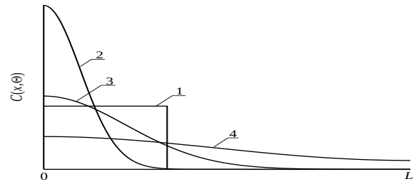
Fig.4a. Distributions of concentration of infused dopant in depth of heterostructure from Fig. 1 for different values of annealing time (curves 2-4) and idealized step-wise approximation (curve 1). Increasing of number of curve corresponds to increasing of annealing time
