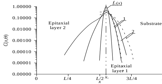
Fig.3b. Calculated distributions of implanted dopant in epitaxial layers of heterostructure. Solid lines are spatial distributions of implanted dopant in system of two epitaxial layers. Dashed lines are spatial distributions of implanted dopant in one epitaxial layer. Annealing time increases with increasing of number of curves
