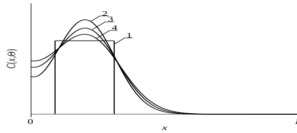
Fig.4b. Distributions of concentration of implanted dopant in depth of heterostructure from Fig. 1 for different values of annealing time (curves 2-4) and idealized step-wise approximation (curve 1). Increasing of number of curve corresponds to increasing of annealing time
