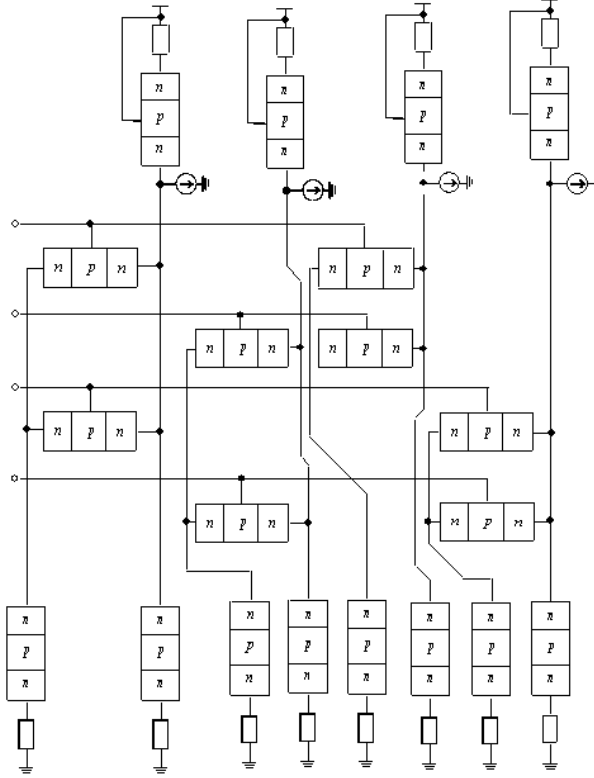
Fig. 1. The considered binary-ROM circuit [4]
