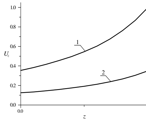
Fig. 8. Normalized dependences of component u_z of displacement vector on coordinate z for nonporous (curve 1) and porous (curve 2) epitaxial layers
