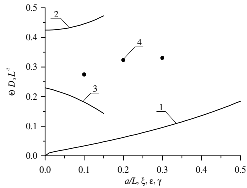
Fig.6. Dependences of dimensionless optimal annealing time for doping by diffusion, which have been obtained by minimization of mean-squared error, on several parameters. Curve 1 is the dependence of dimensionless optimal annealing time on the relation a/L and \xi = \gamma = 0 for equal to each other values of dopant diffusion coefficient in all parts of heterostructure. Curve 2 is the dependence of dimensionless optimal annealing time on value of parameter \epsilon for a/L=1/2 and \xi = \gamma = 0 . Curve 3 is the dependence of dimensionless optimal annealing time on value of parameter \xi for a/L=1/2 and \epsilon = \gamma = 0 . Curve 4 is the dependence of dimensionless optimal annealing time on value of parameter \gamma for a/L=1/2 and \epsilon = \xi = 0
