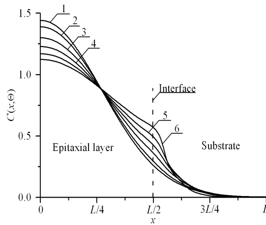
Fig.2. Distributions of concentration of infused dopant in heterostructure from Fig. 1 in direction, which is perpendicular to interface between epitaxial layer substrate. Increasing of number of curve corresponds to increasing of difference between values of dopant diffusion coefficient in layers of heterostructure under condition, when value of dopant diffusion coefficient in epitaxial layer is larger, than value of dopant diffusion coefficient in substrate
