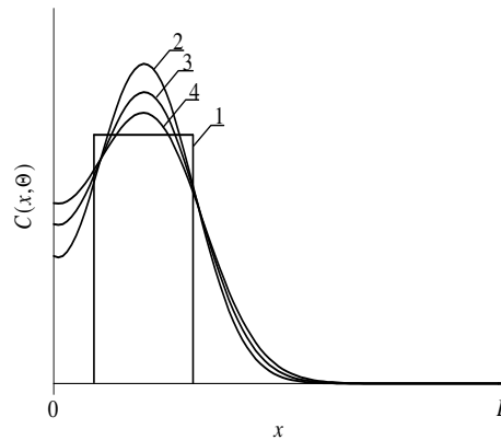
Fig. 5. Spatial distributions of dopant in heterostructure after ion implantation. Curve 1 is idealized distribution of dopant. Curves 2-4 are real distributions of dopant for different values of annealing time. Increasing of number of curve corresponds to increasing of annealing time
