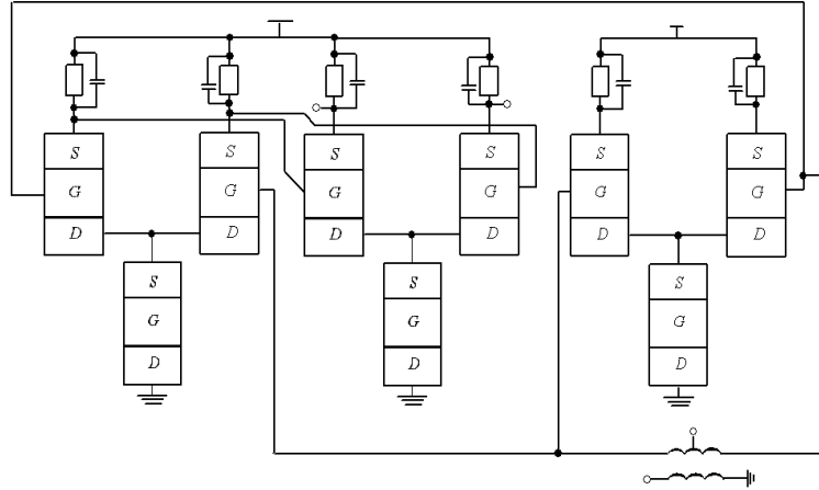
Fig. 1a. Structure of the considered voltage reference [20]
