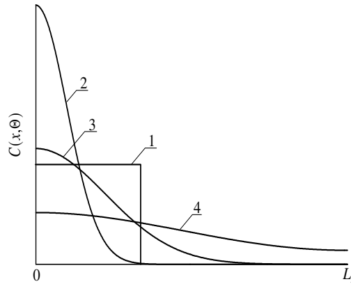
Fig. 4. Spatial distributions of dopant in heterostructure after dopant infusion. Curve 1 is idealized distribution of dopant. Curves 2-4 are real distributions of dopant for different values of annealing time. Increasing of number of curve corresponds to increasing of annealing time
