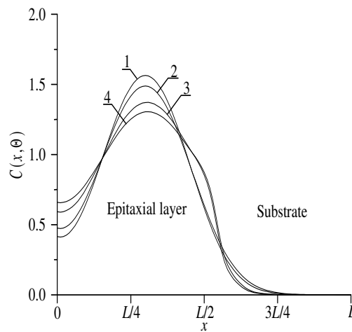
Fig.3. Distributions of concentration of implanted dopant in heterostructure from Fig. 1 in direction, which is perpendicular to interface between epitaxial layer substrate. Curves 1 and 3 corresponds to annealing time \Theta = 0.0048(L_x^2 + L_y^2 + L_z^2)/D_0 . Curves 2 and 4 corresponds to annealing time \Theta = 0.0057(L_x^2 + L_y^2 + L_z^2)/D_0 . Curves 1 and 2 corresponds to homogenous sample. Curves 3 and 4 corresponds to heterostructure under condition, when value of dopant diffusion coefficient in epitaxial layer is larger, than value of dopant diffusion coefficient in substrate
