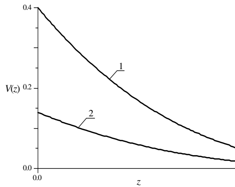
Fig. 9. Normalized dependences of vacancy concentrations on coordinate z in unstressed (curve 1) and stressed (curve 2) epitaxial layers
