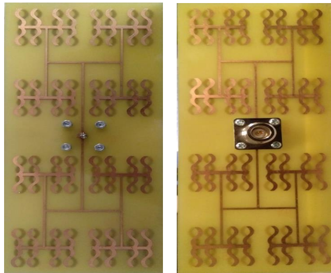
(c) 4x4 Array Varians.
