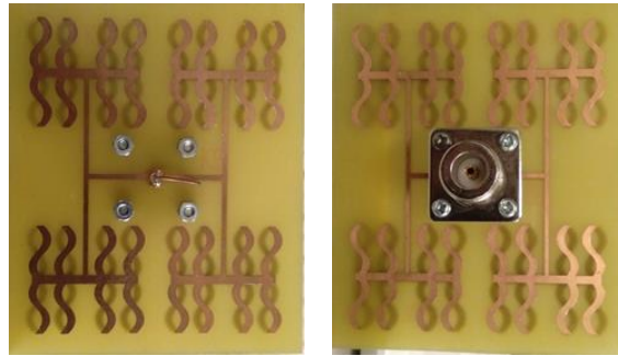
(b) 2x4 Array Varians.
