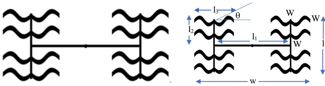
Figure 1. (a) Curved Microstripline 2x2 Array Antenna Design (b) Dimension of Curved Microstripline 2x2 Array Antenna Design.
