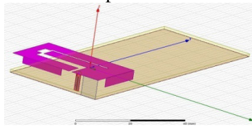
Fig 3. PIFA design
