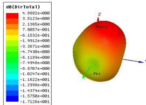
Fig 14. Directivity plot for f_r = 1.93\text{GHz}
