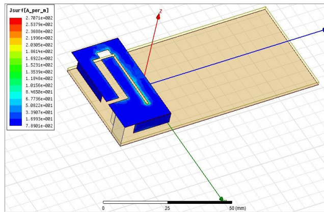
Fig 15 (a): Surface current distribution at 0.89GHz
