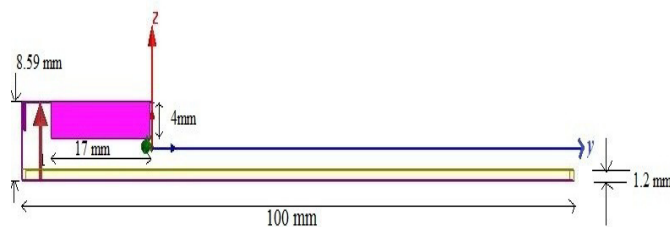
Fig 6. Side View
