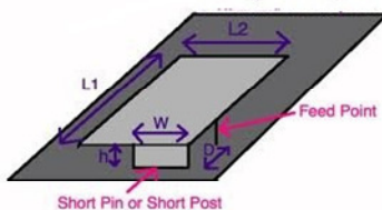
Fig 2. Basic PIFA
