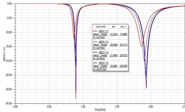
Fig 9: Variation of return loss with frequency for different short plane width
