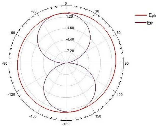
Fig 11. Radiation pattern for f_r = 0.89\text{GHz}
