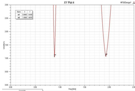
Fig 8. VSWR of PIFA
