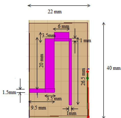
Fig 4. Top view of PIFA
