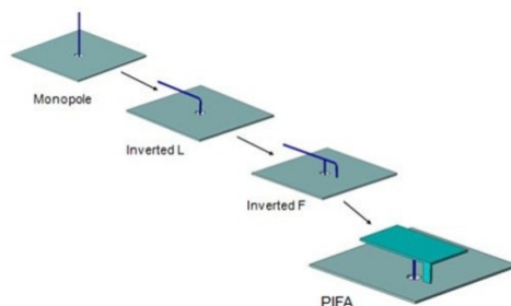
Fig 1. PIFA from monopole
