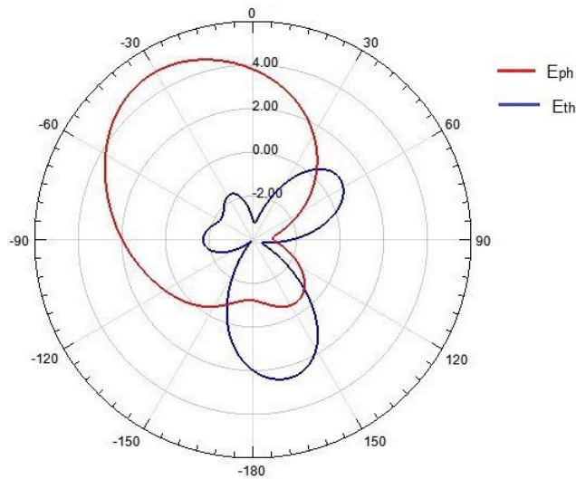
Fig 12. Radiation pattern for f_r = 1.93\text{GHz}
