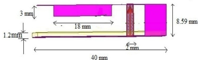
Fig 5. Front View
