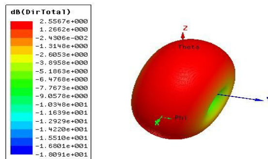
Fig 13. Directivity plot for f_r = 0.89\text{GHz}
