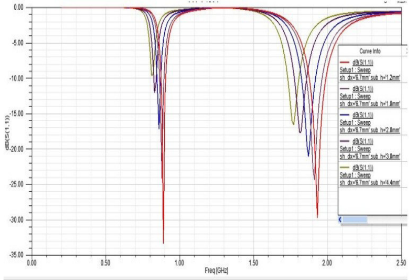
Fig 10. Return loss corresponding to substrate height variation
