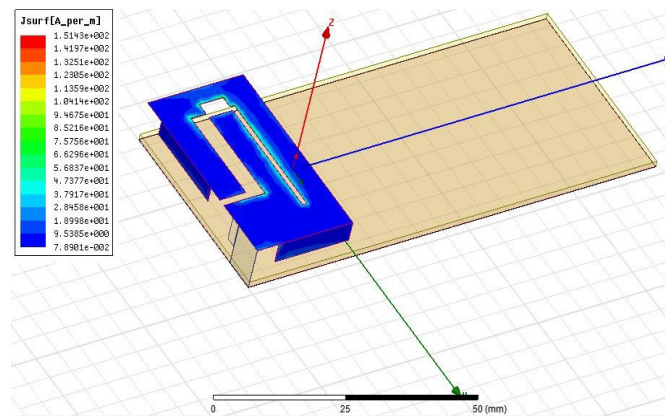
Fig 15 (b): Surface current distribution at 1.93GHz
