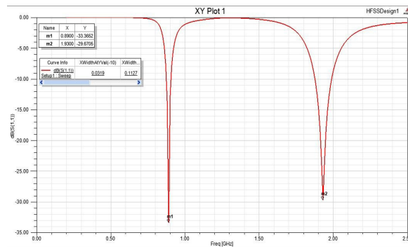
Fig 7. Return loss of PIFA
