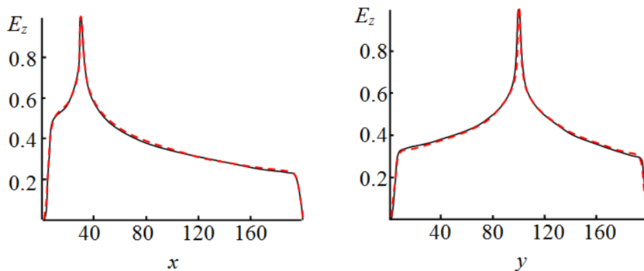
Fig.2 Projections of the field distribution E(x,y) inside 2D area (Fig.1a) on the plane of two variables ( E,x ) (a) and ( E,y ) (b).
