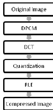
Figure 3. The steps of the proposed method
