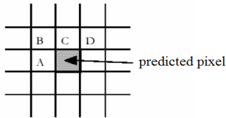
Figure 1. Predictor Model
