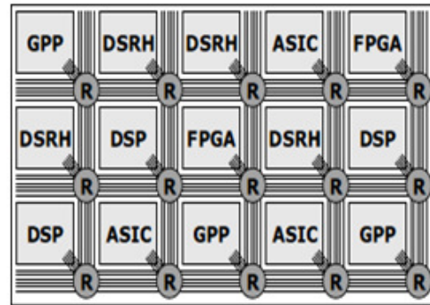
Fig 2. An Example of a Heterogeneous System-on-Chip (SoC) with a Network-on-Chip (NoC)
