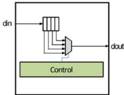
Fig 3. Input FIFO for Original Router
