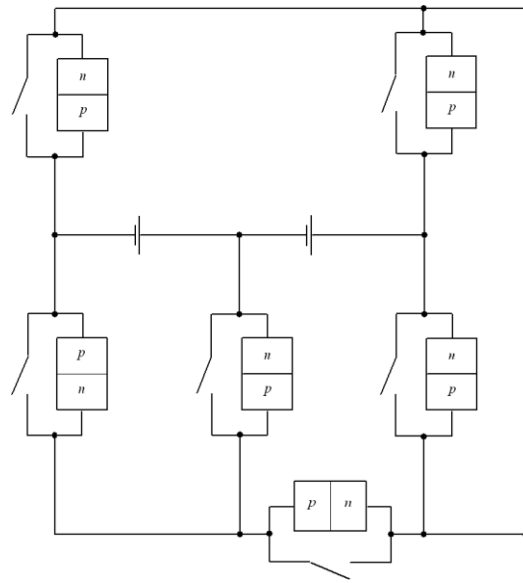
Fig. 1a. Structure of the considered inverter [15]
